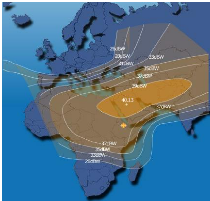
PAKSAT 1 at 38,0°East – northern BEAM – point of reception Slovakia
