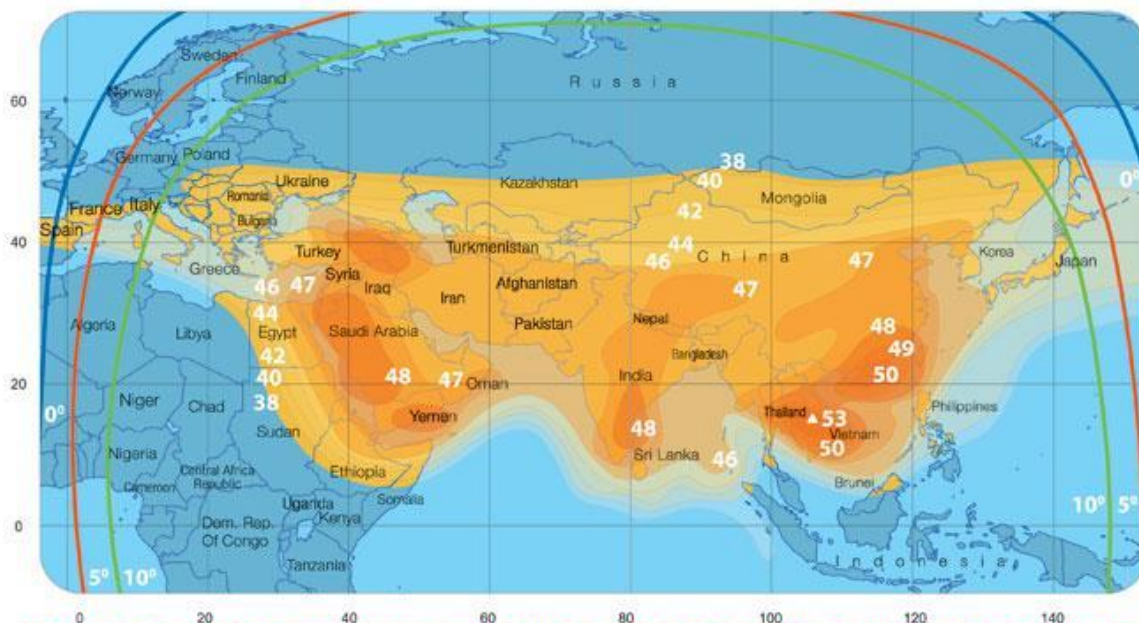
tp 12S - Southern beam : recommend dish diameter in central Europe : 180-270+ cm
