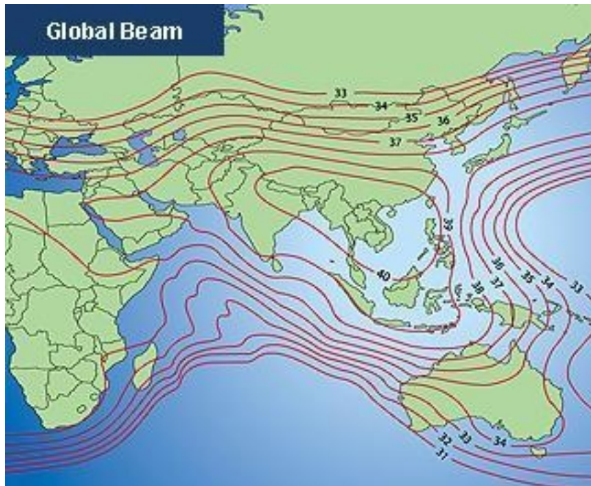
Measat 3 at 91,5°E – Global C footprint
