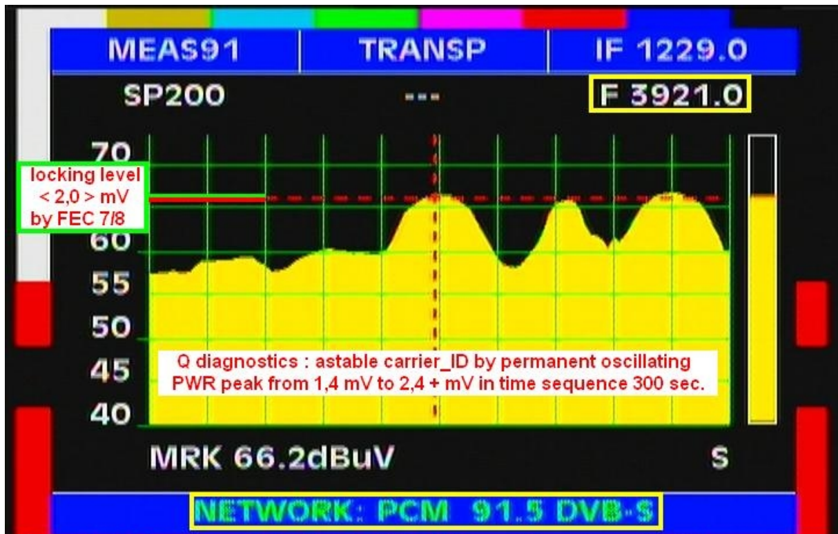
Measat 3 at 91,5°E - Global C SPOT : 3 921 V PCM Network Hong Kong_TP 11C spectral scan
