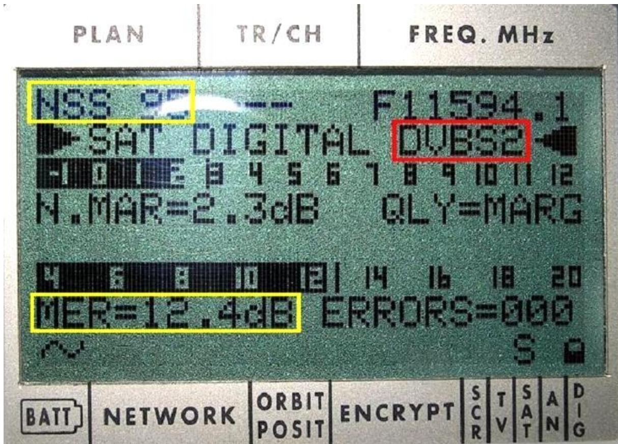
Reception quality & DVB-S2_PER diagnostics
