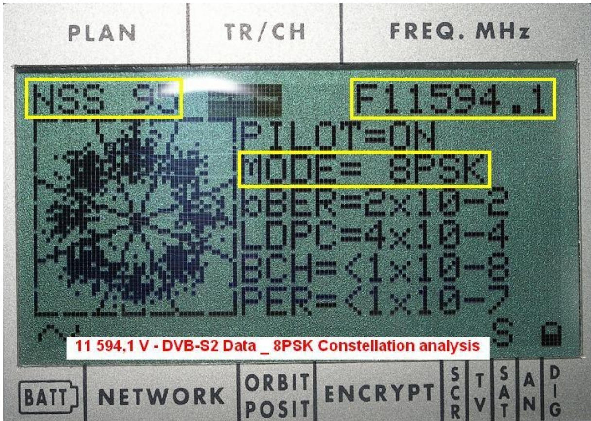
Constellation analysis : modulation 8PSK
