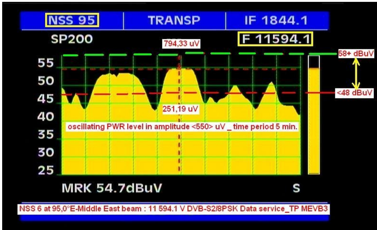
Spectral analysis & reception condition
